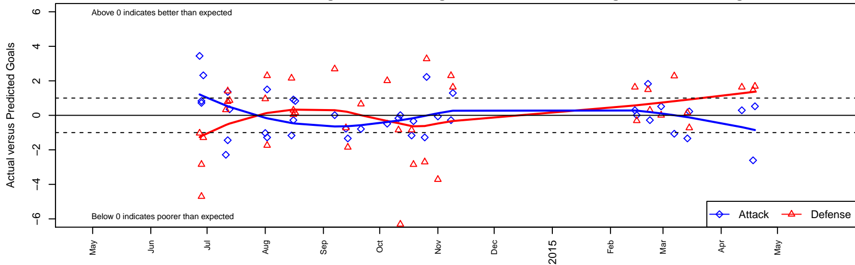
ETFC Ajax Black –was Blue B03 Dots are actual minus expected GF (blue circles) and GA (red triangles). Blue line is smoothed change in attack strength. Red is smoothed change in defense strength.
